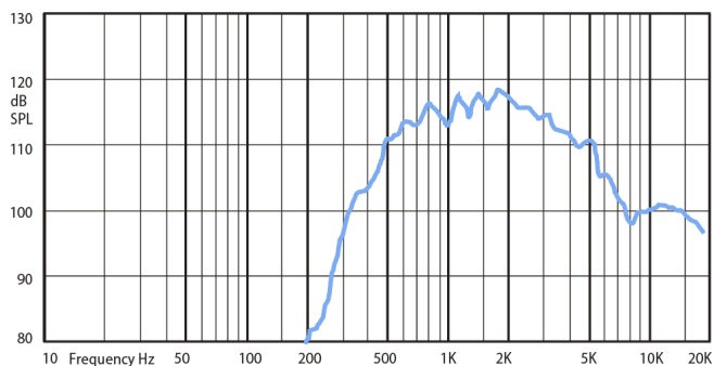
Frequency response
