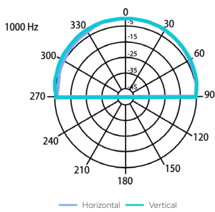
Horizontal/vertical polar diagrams
